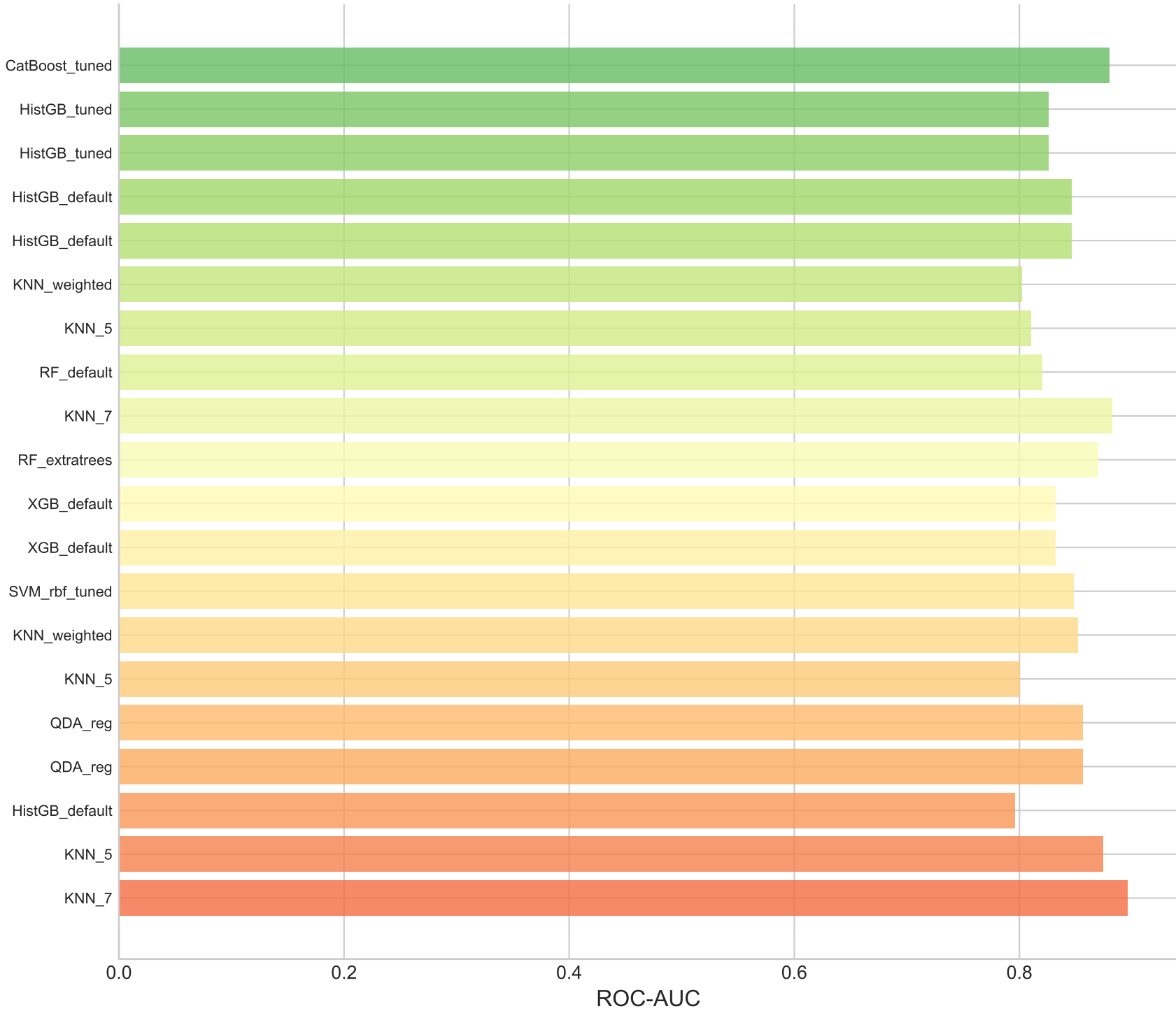
Top 20 Models - ROC-AUC (Two-Class)
