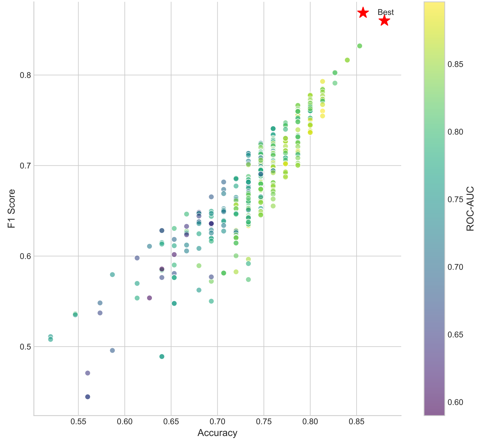
Accuracy vs F1 Score (colored by ROC-AUC) - Two-Class
